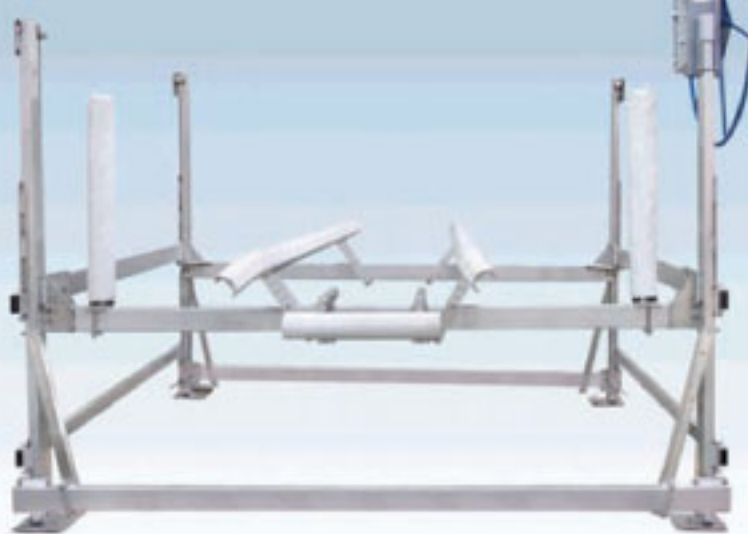
VL with Pivoting Aluminum & Vinyl Bunks, Aluminum & Vinyl Motor Stop and Vertical Guide Posts
